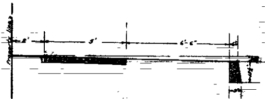
SECTION OF SIDEWALK AND CURB AT A-A SCALE 1/2"=1'
